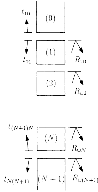
Fig. 2. Configuration to calculate the total reflection coefficients recursively.
